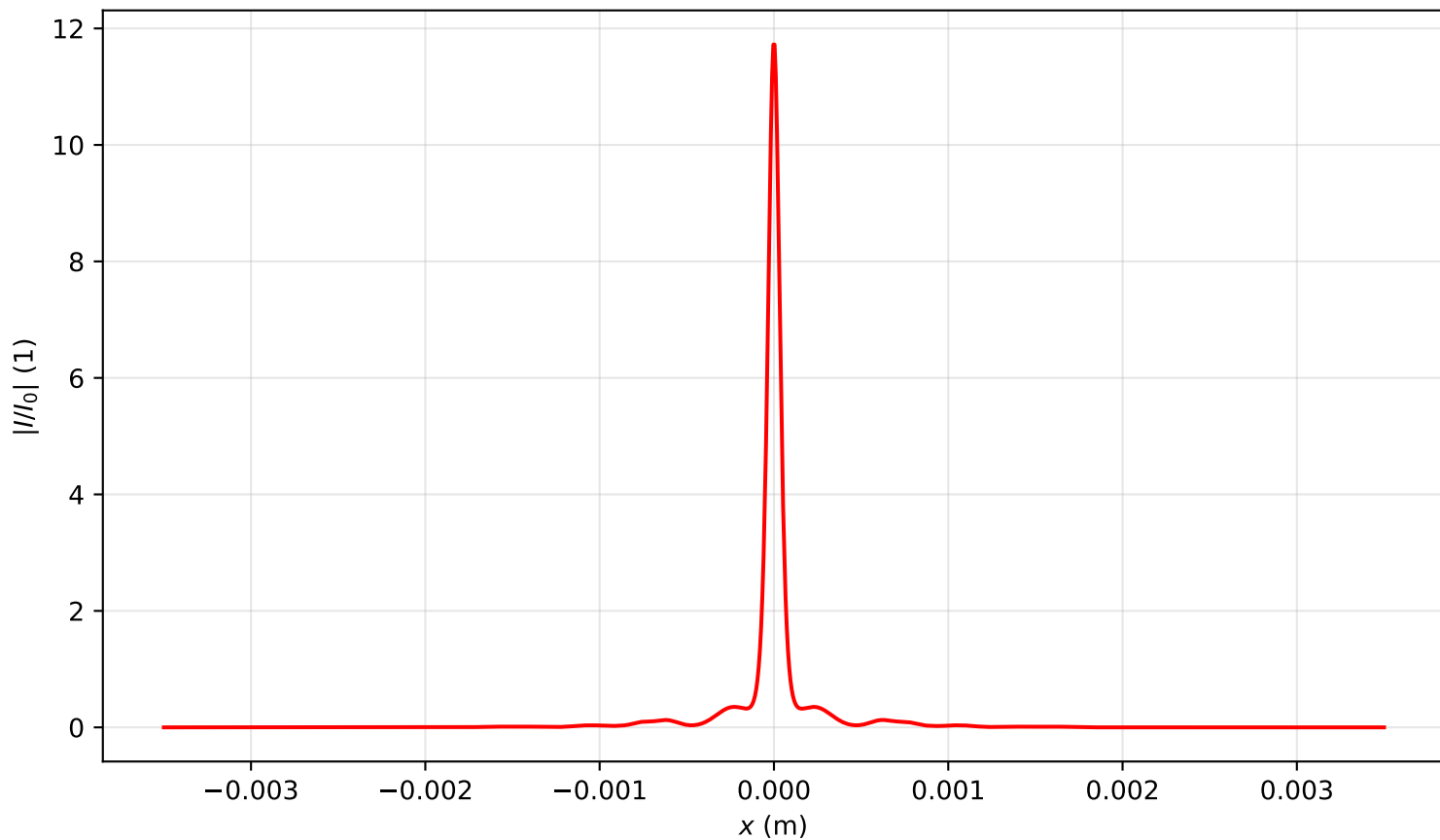
Intensity profile I(x, y = 0, z = 1.433)/I_0 , P_{in}=6.5P_{cr} , artificial time
